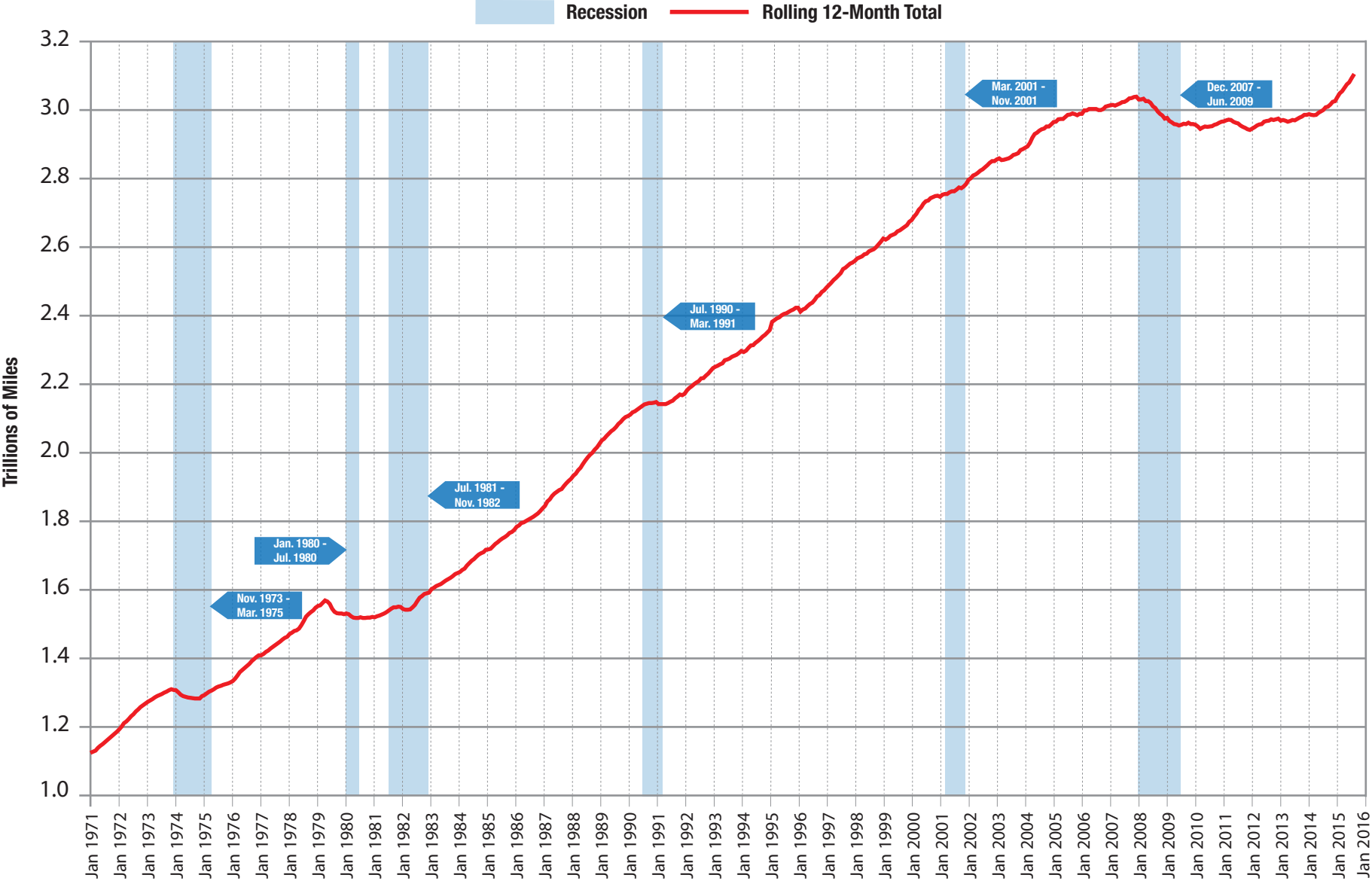
U.S. Vehicle Miles Traveled Rolling 12-Month Total, All Roads
